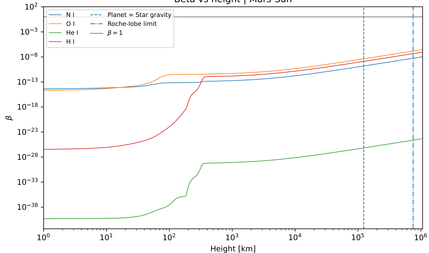
Beta vs height | Mars-Sun
